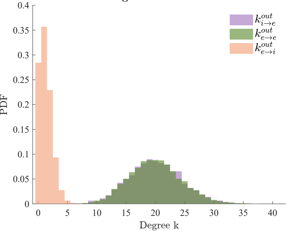
Degree Distribution
